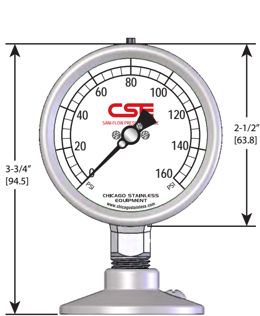
2-1/2" BOTTOM MOUNT (Shown with 1-1/2" Tri-Clamp)
