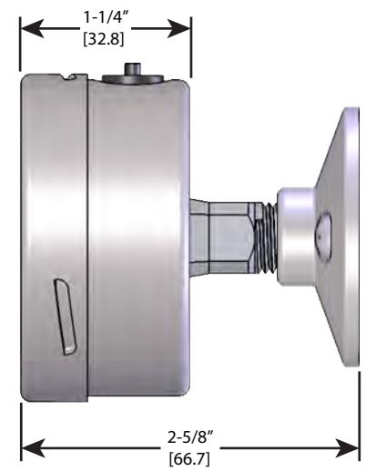
2-1/2" BACK MOUNT (Shown with 1-1/2" Tri-Clamp)
