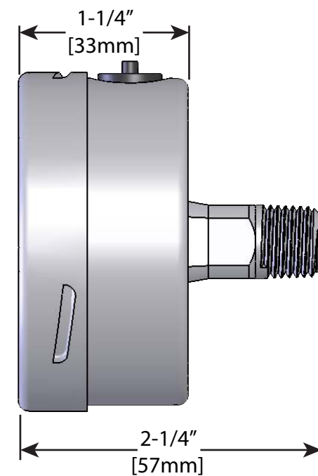
2-1/2" BACK MOUNT
