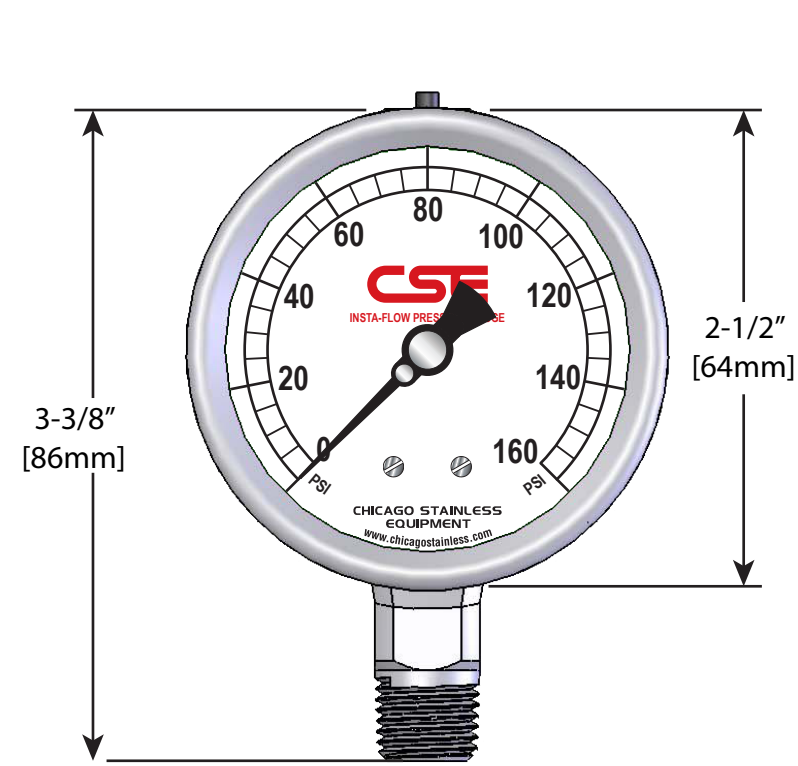
2-1/2" BOTTOM MOUNT
