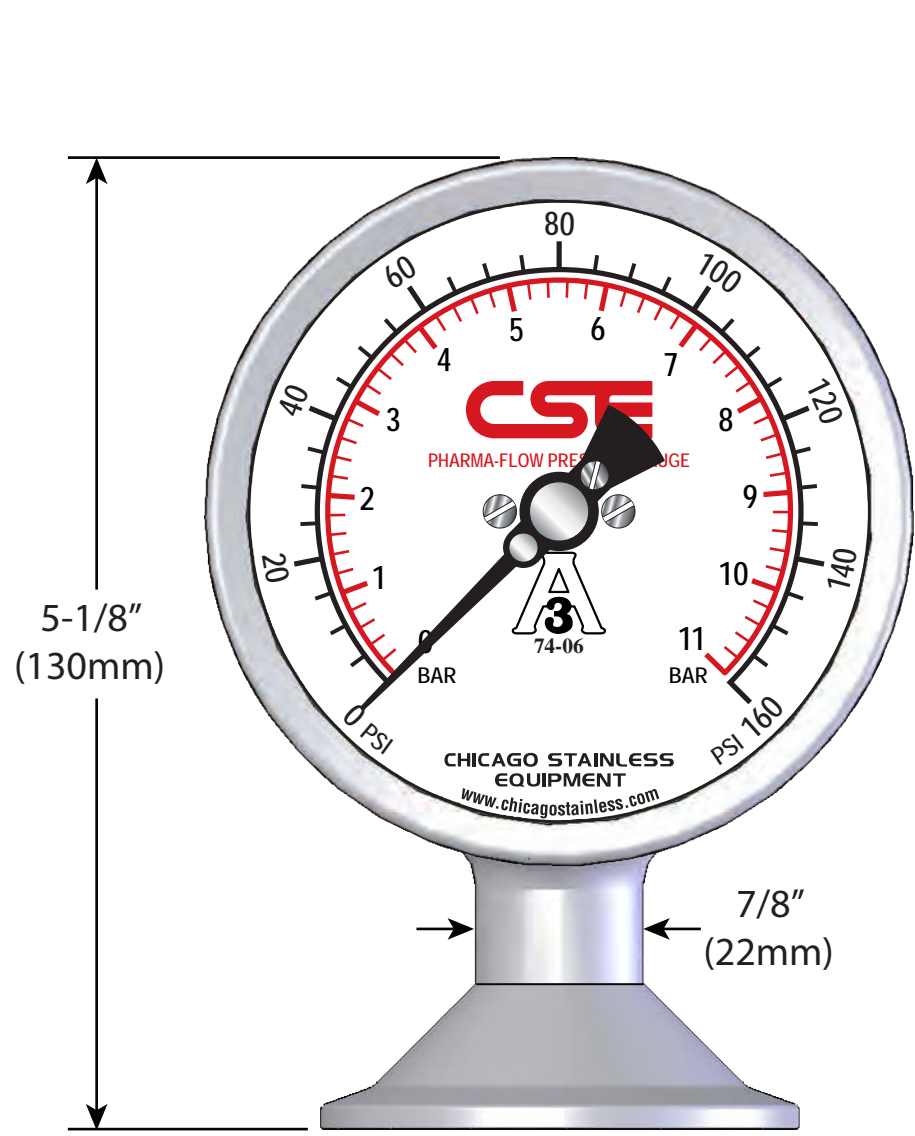
3-1/2" BOTTOM MOUNT (Shown with 2" Tri-Clamp)
